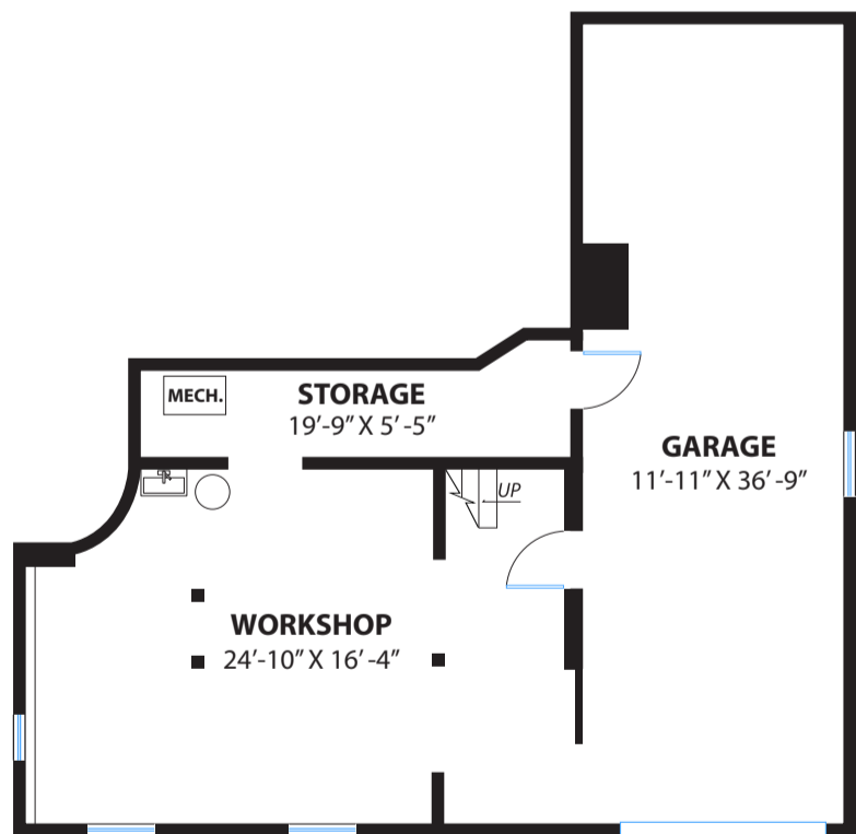
GARAGE/ BASEMENT LEVEL
